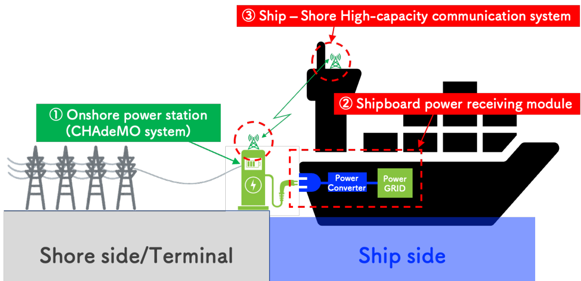
Figure 1 : Configuration image of Standard universal zero emission charger system for ships
