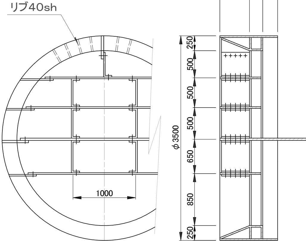
呼び径3000mm
